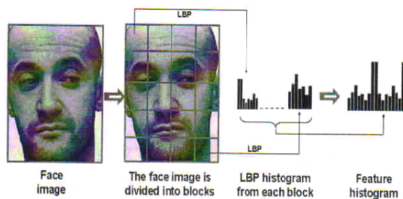
Fig.2 Examples of an LBP based facial representation
