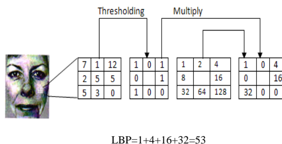
Fig 1.Example of an LBP calculation
